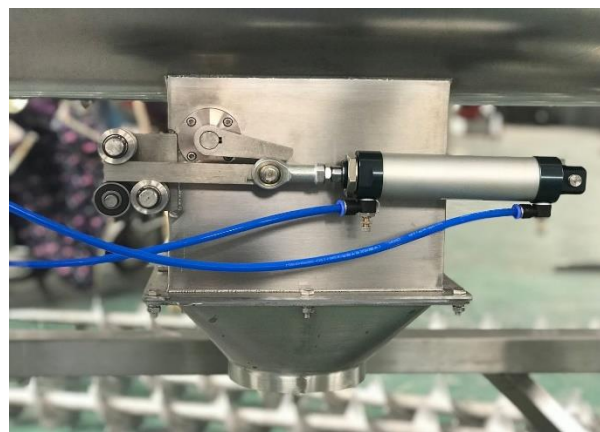
The pneumatic discharging device
